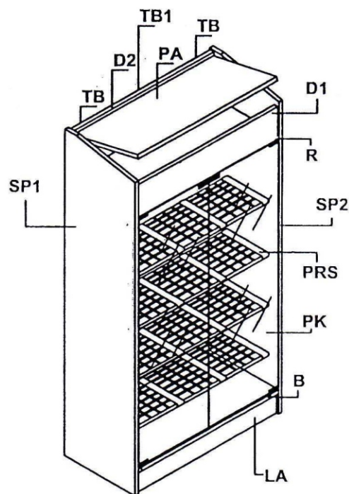
FINAL ASSEMBLING
